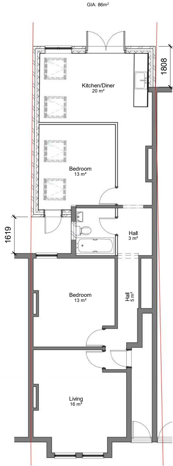
Proposed GFL 1 : 100
